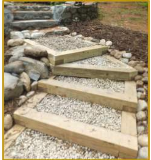
Infiltration Steps - Crushed stone steps that trap stormwater instead of allowing it to flow downhill.
