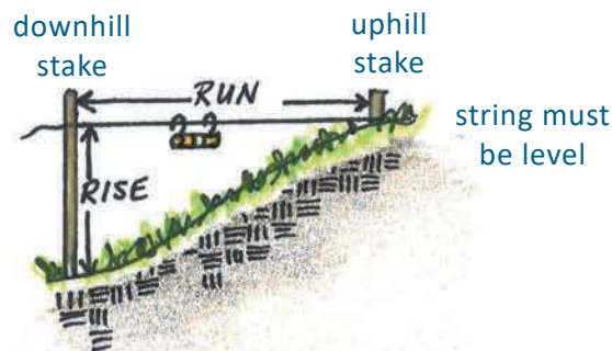
Figure 2 – Determine the slope of the landscape before digging.
