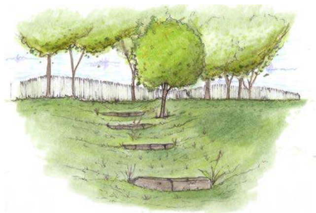
Figure 2. Check dams within a swale slow the flow, allowing sediments to settle out and some infiltration to occur.
